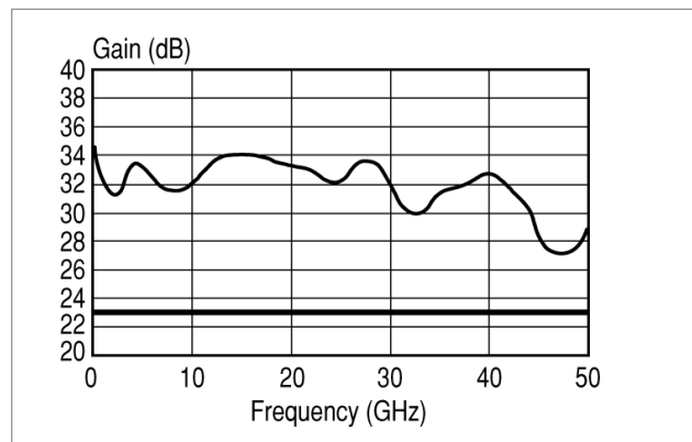
Gain of 83051A amplifier
