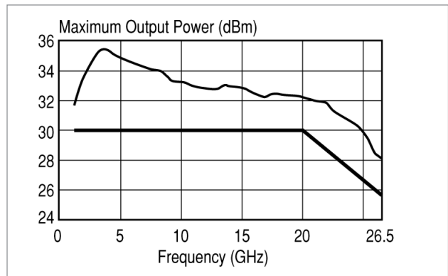
Max Output Power of 83020A amplifier
